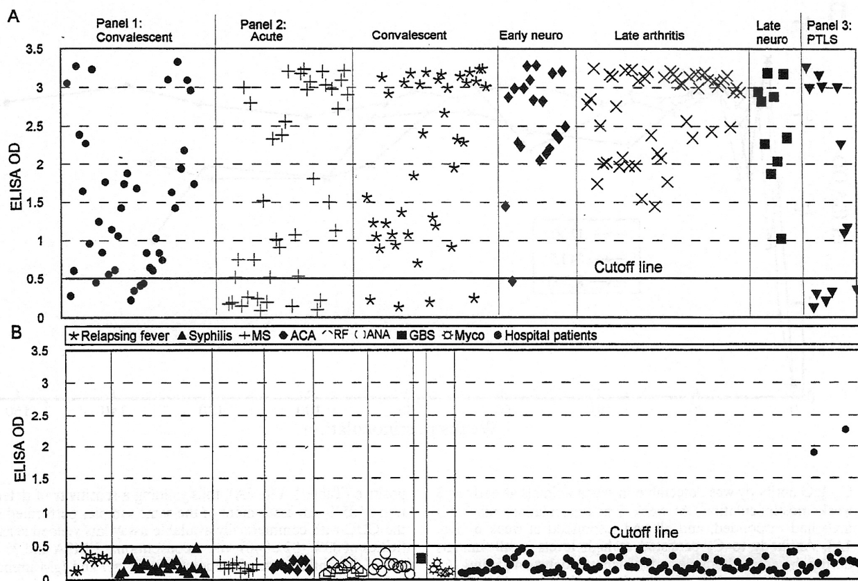
FIG. 2. Assessment of sensitivity (A) and specificity (B) of the C 6 ELISA. (A) Three panels of serum samples from patients with Lyme disease were tested with the C 6 ELISA at a serum dilution of 1:200. Panel 1 was composed of specimens collected during the convalescent phase; panel 2 was composed of samples from the acute, convalescent, early disseminated (early neuroborreliosis [neuro]), and late (arthritis and neuroborreliosis [neuro]) phases; and panel 3 was composed of samples from patients with posttreatment Lyme disease syndrome (PTLS). (B) Specimens were from patients with relapsing fever, syphilis, multiple sclerosis (MS), positive anticardiolipin antibody (ACA), positive rheumatoid factor (RF), positive antinuclear antibody (ANA), Guillain-Barré syndrome (GBS), or mycobacterial infection (Myco). In addition, 99 serum specimens from patients of a hospital in Louisiana, where Lyme disease is not endemic, were tested; the cutoff OD value (0.500) was defined as the mean plus 3 SDs for 97 serum samples from this panel.
