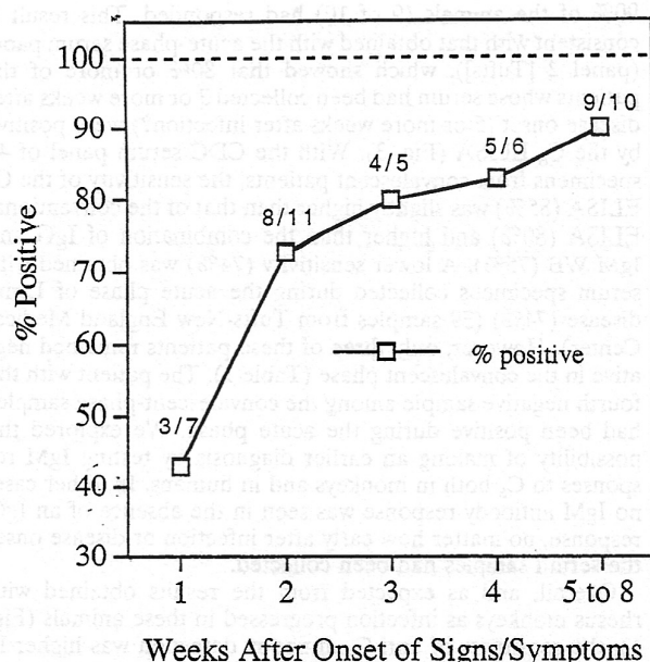
FIG. 3. Fraction of positive samples as a function of time after disease onset. The anti- C_6 antibody-positive fraction of serum samples obtained at consecutive weeks after the onset of signs or symptoms is shown. The acute-phase group of serum specimens from panel 2 was used at a dilution of 1:200.
